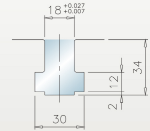
V-1200 T-Slot dimensions
