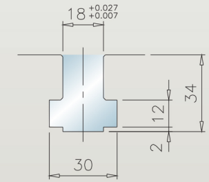
V-1400N T-Slot dimensions
